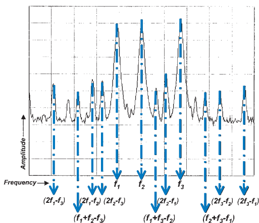
Figure 3-6: three-transmitter intermodulation
