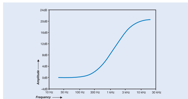
Figure 2-4a: pre-emphasis in transmitter
