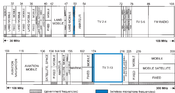
Figure 3-2: VHF allocations in the United States (30-300 MHz)
