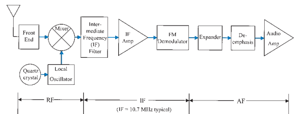
Figure 2-11b: single conversion, frequency-synthesized receiver
