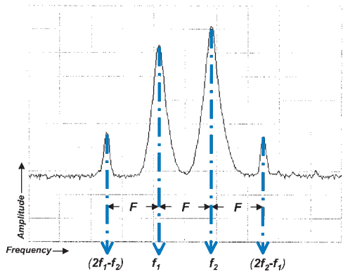
Figure 3-5: two-transmitter intermodulation
