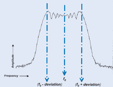
Figure 2-6b: modulated FM signal spectrum
