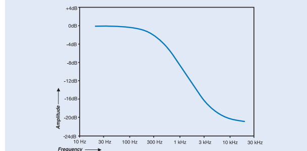
Figure 2-4b: de-emphasis in transmitter
