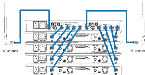
Figure 2-32a: active antenna distribution (one level)
