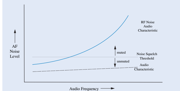
Figure 2-15: noise squelch
