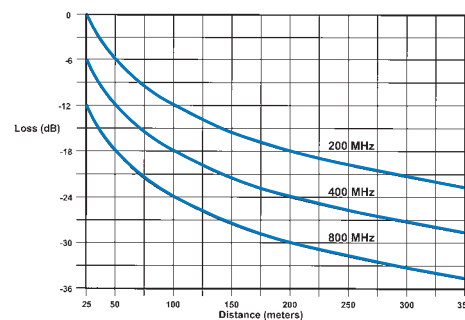
Figure 3-15: loss vs. distance vs. frequency
