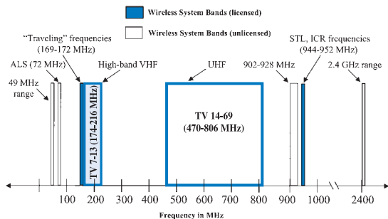
Figure 3-1: wireless frequency bands in the United States
