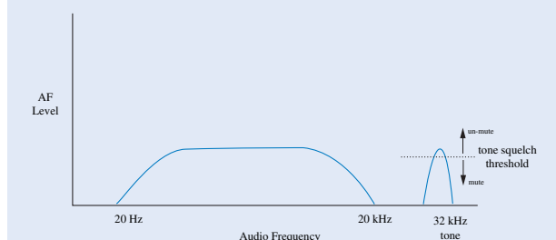
Figure 2-16: tone key squelch
